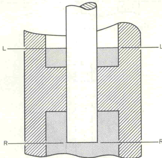
FIGURE 1. Piston of uniform cross section
